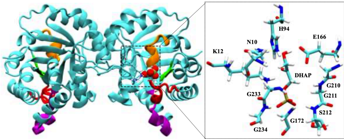
Figure 1: Structure of TIM dimer with DHAP in the active site. Loop-6 (red), loop-7 (green) and loop-8 (orange) envelope the active site. Loop-5 (purple) interacts with N-terminus residues of loop-6. In inset residues of the active site which are highly conserved.
